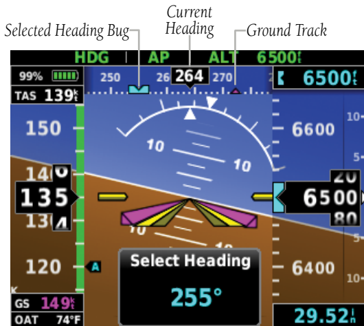
Figure 2-12 PFD Page - Selected Heading
